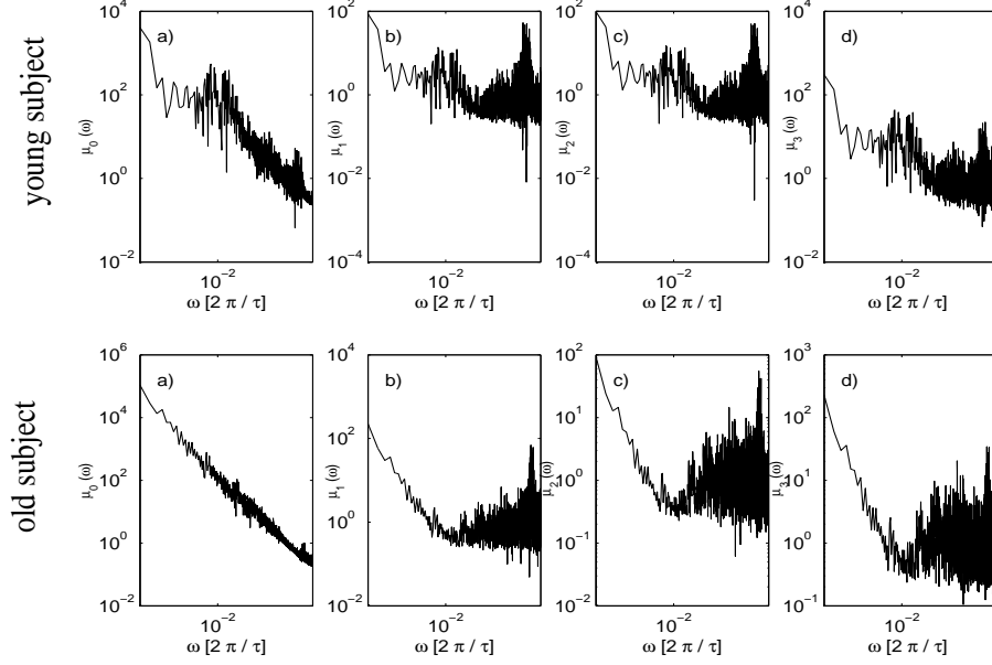
Figure 3: The power spectra of the initial TCF (a) and the first three memory functions (b-d) for the young and elderly persons. The power spectra of the initial TCF of the elderly person differs in smaller dynamic breaks in the field of low frequencies. In all the power spectra the dynamic splashes (peaks) are found in the field of high frequencies, which is connected with respiratory arrhythmia. These dynamic peaks of the elderly person are shifted in the area of higher frequencies. It testifies to the increase in frequency of cardiac reductions at breath that comes with ageing.
